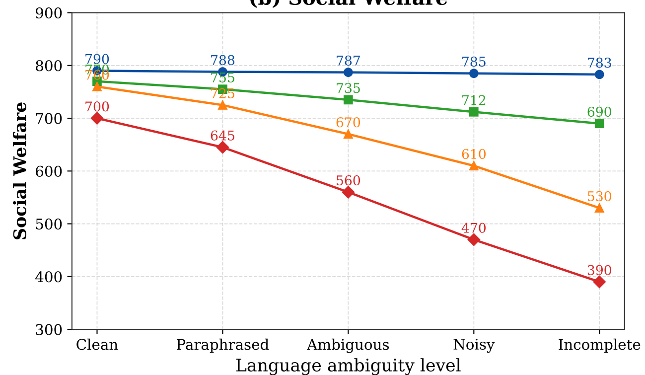
(b) Social Welfare
